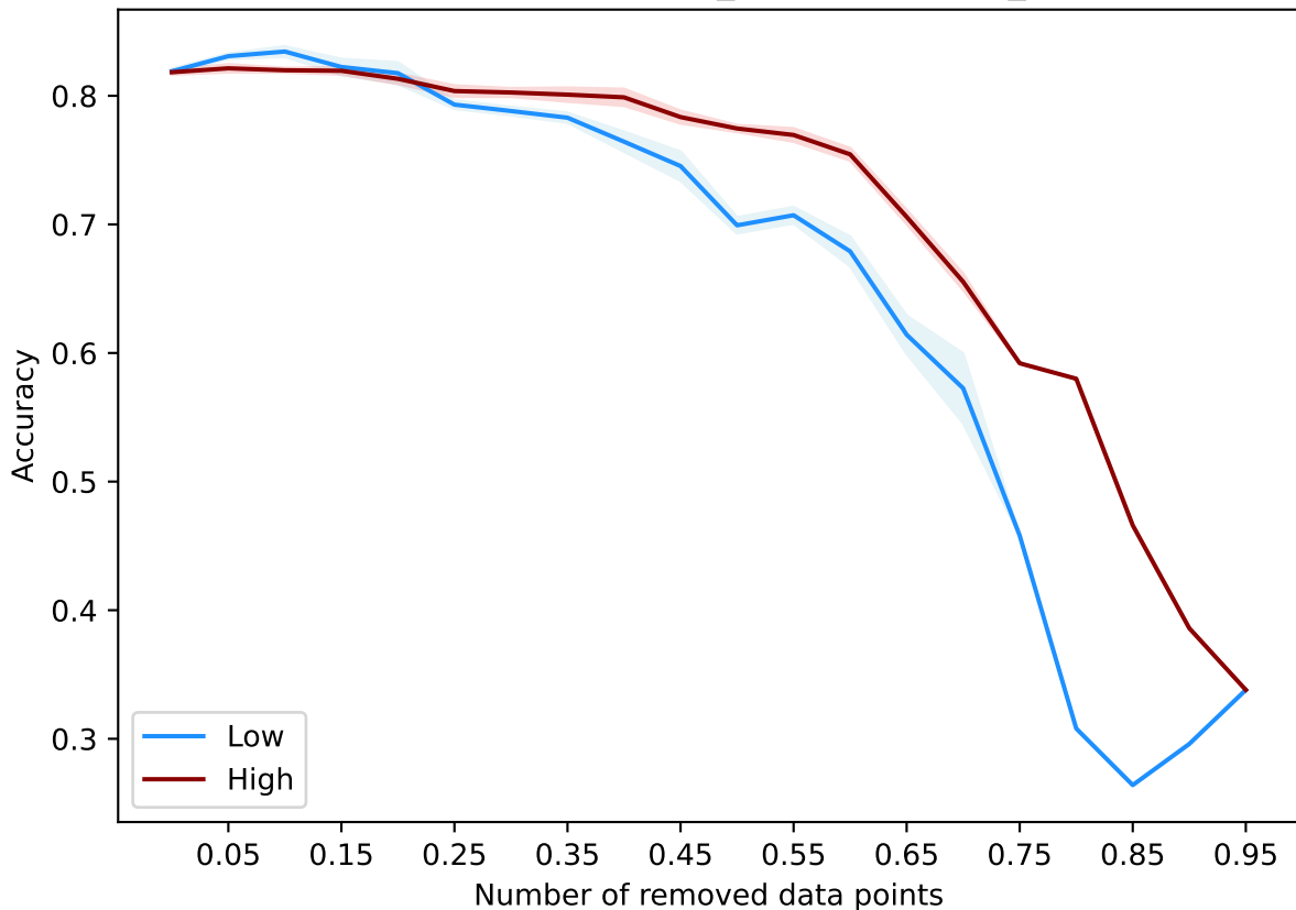
PruningOptimization(optimization_type=size, only_size=300) - pol
